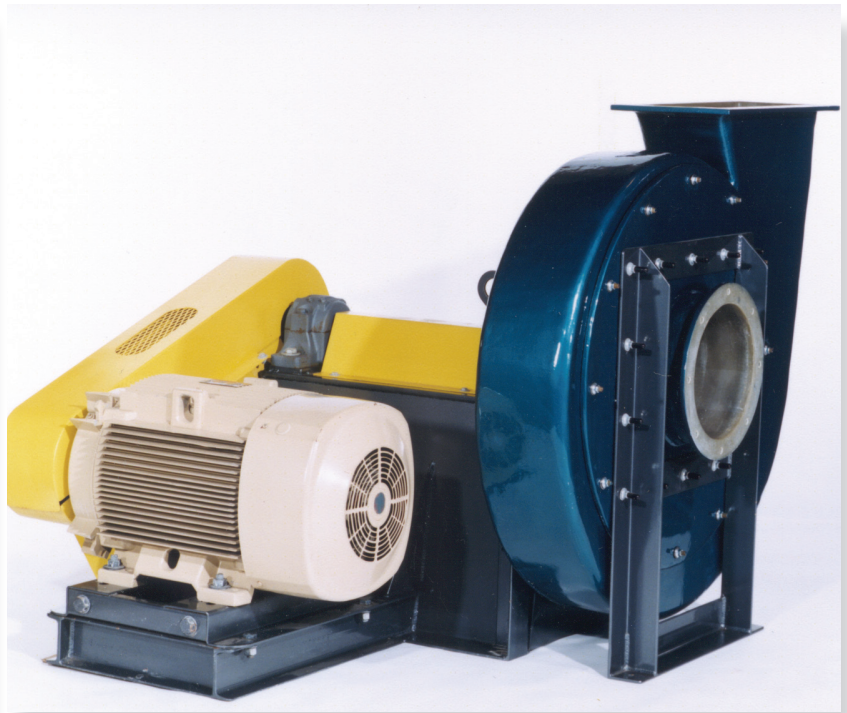
Standard catalog type HP arrangement 4 fan with pie split housing (left). Belt drive arrangement 9F (right).
